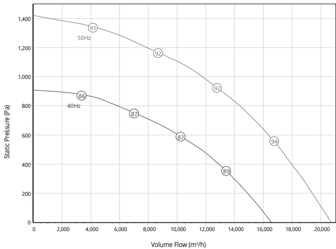
ESTOC TARGE 102-630-3 - GF163027
