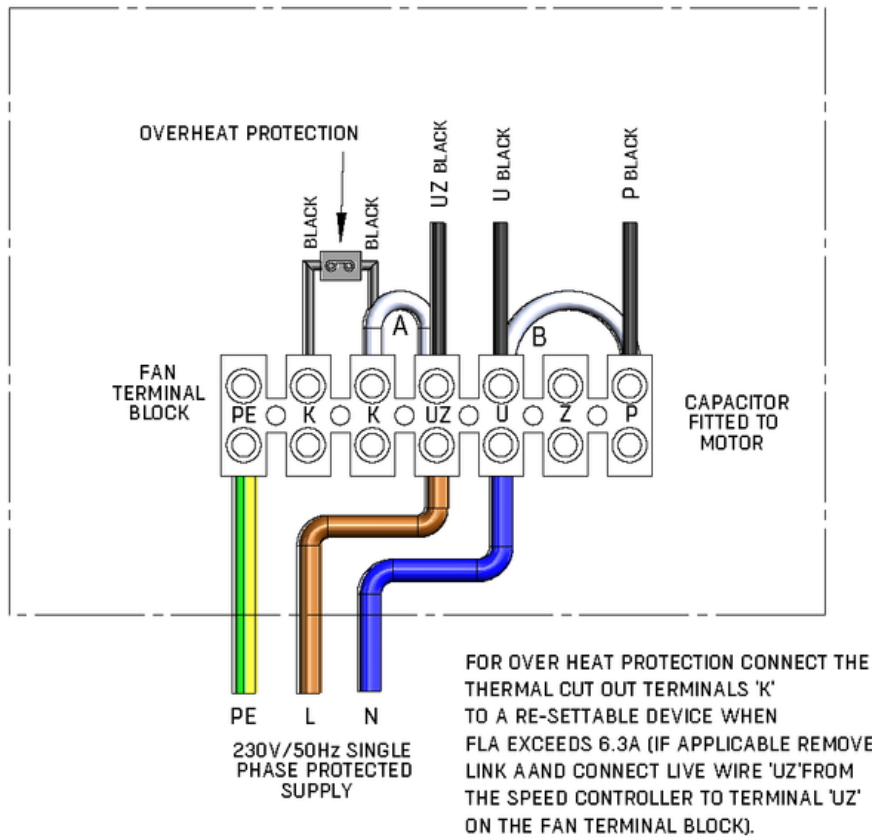
FAN CONNECTED TO SUPPLY (FULL SPEED)
